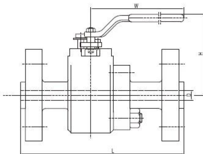
Full Port (1/2"~2")
