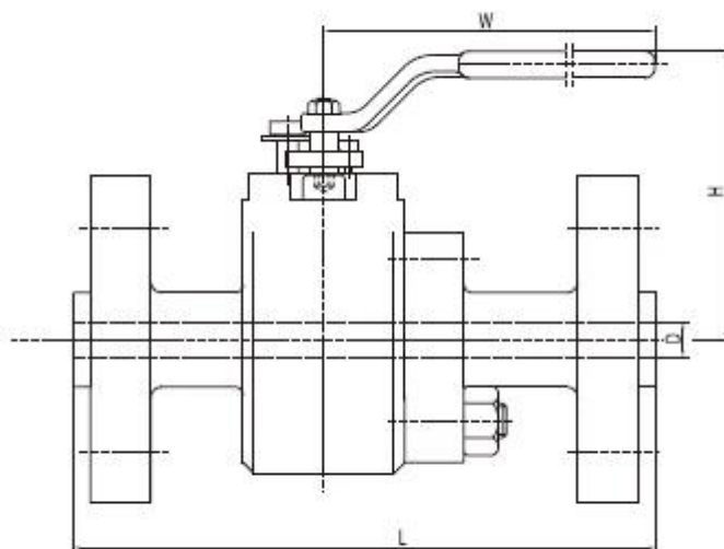
Full Port (1/2"-2")
